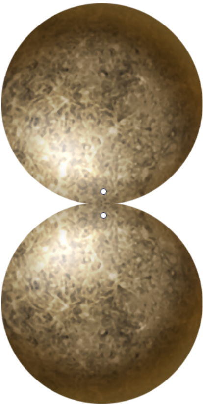
Mercure
