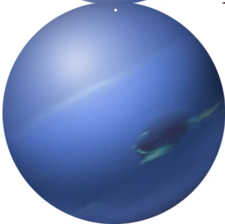
Neptune
